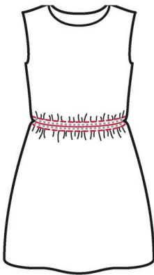
ALTERNATIVE CASING USING A SEAM ALLOWANCE (p.158)
